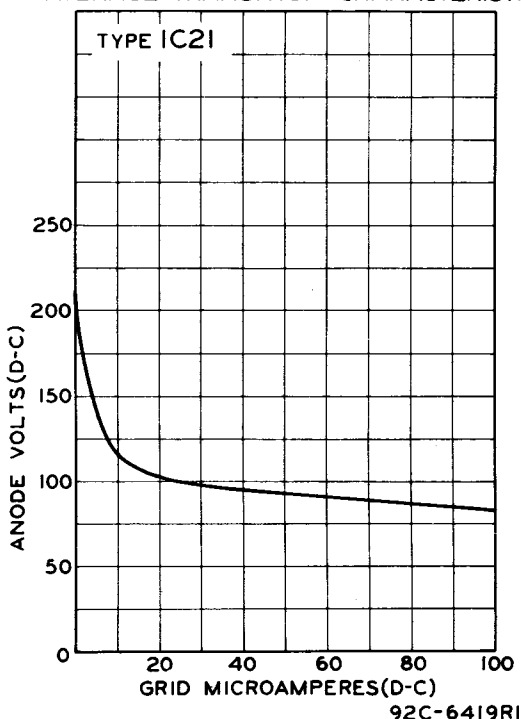
AVERAGE TRANSITION CHARACTERISTIC
