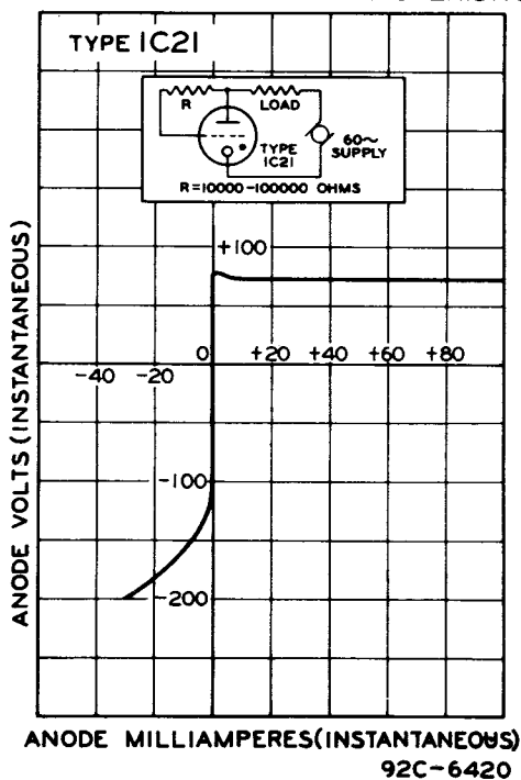
AVERAGE ANODE CHARACTERISTIC
